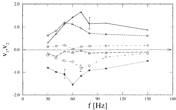
FIG. 2. Average vertical components of the velocity in the center ( v_1 ) and the sides ( v_2 ) of the cell as function of the frequency f for amplitudes A_0 = 0.7d_0 (+ for v_1 and * for v_2 ), A_0 = 0.5d_0 (x for v_1 and o for v_2 ), and A_0 = 0.3d_0 (◇ for v_1 and △ for v_2 ). All other parameters are as in Fig. 1.
