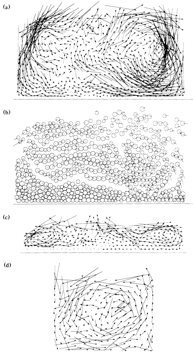
FIG. 3. Convection cells due to fixed vertical walls for B = 0 , w = 0.5 , Y = 5000/d_0 . (a) Displacements after eight cycles and (b) snapshot of the positions of the particles for f = 20 Hz, N = 600 , L = 46d_0 , A_0 = 1.25d_0 , \gamma = 80g , \gamma_s = 100g ; (c) f = 20 Hz, N = 300 , L = 44d_0 , A_0 = 1.1d_0 , \gamma = 80g , \gamma_s = 100g , averaged over ten cycles; (d) f = 100 Hz, N = 200 , L = 20d_0 , A_0 = 0.5d_0 , \gamma = 50g , \gamma_s = 0 , averaged over fifteen cycles.
